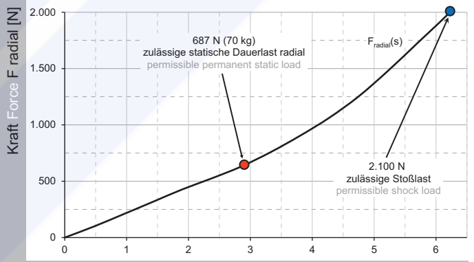
Federweg Spring deflection s radial [mm]
